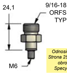
90.505.116 (S-116) M6 → 9/16-18
