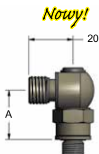
90.807.230 90°Adapter Portu
