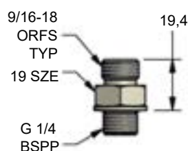
90.505.122 (S-122) Prosto
