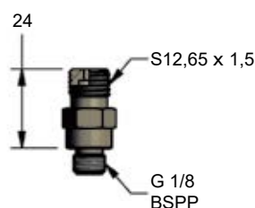
90.805.115 Prosty Adapter Portu
