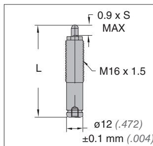
Basic dimensions
