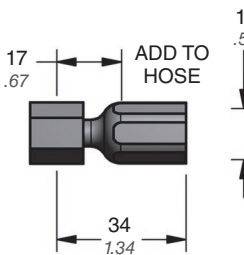
90.508.843 (D-843) Compact Hose Adapter
