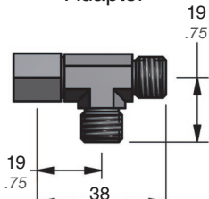
90.508.432 (D-432) Run Tee
