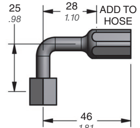
90.508.858 (D-858) 90° Hose Adapter
