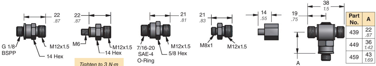
90.508.115 (D-115) Straight Port Adapter
