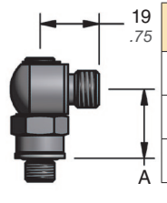
90.508.230 (D-230) 90° Branch Tee
